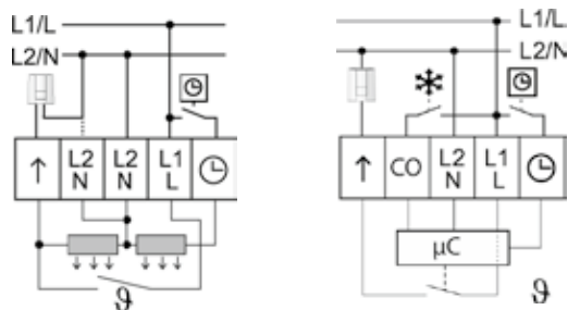
Schaltplan RT-A
