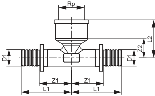
TECEflex tee female thread
