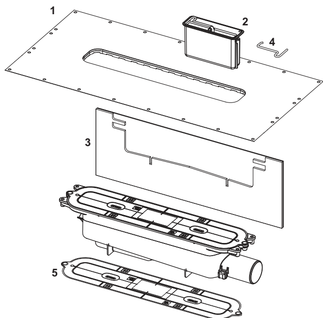
TECEdrainprofile standartinis sifonas DN 50, šoninis pajungimas
