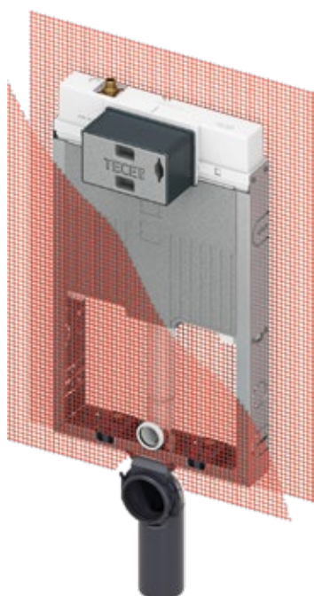
TECEbox toilet module with Octa cistern, 8 cm, for wall toilet, installation height 1075 mm.
