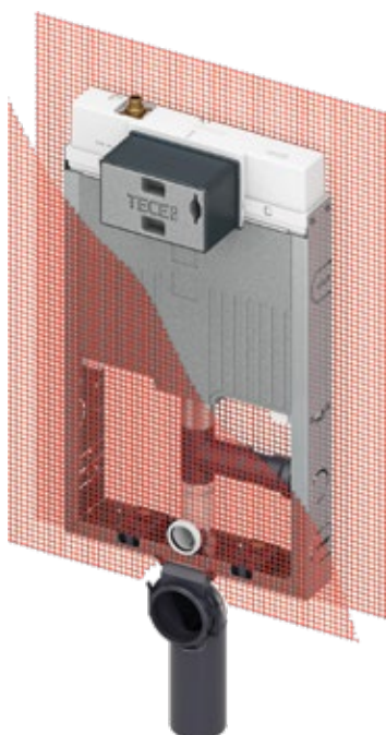
TECEbox toilet module with Uni cistern, 8 cm, with connection for odour extraction, installation height 1075 mm.
