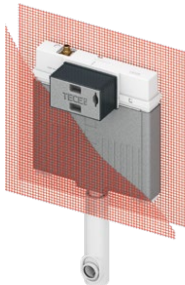
TECEbox Octa cistern, 8 cm, for standing toilet, with reinforcement fabric, installation height 1075 mm.
