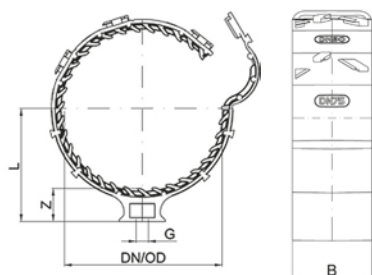
POLO-CLIP HS (FIGUR 6)
