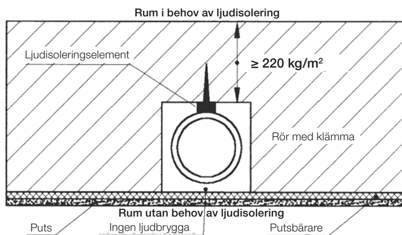
Konventionell installation (FIGUR 28)
