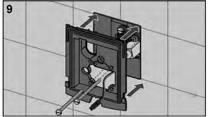
Screw the support frame onto the urinal flush valve housing.
