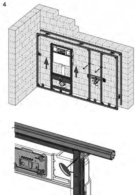
Pull out the module, secure it with corner joints on the upper profiled tube, apply the foot brake, tighten the screws on the module feet (only by hand!)
