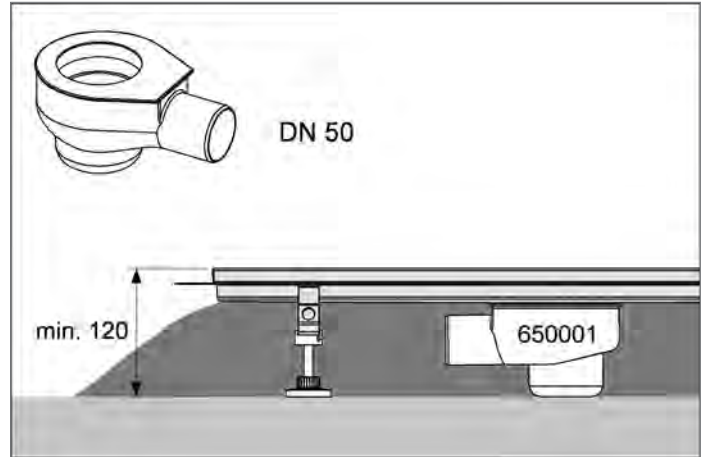
"Standard" outlet
