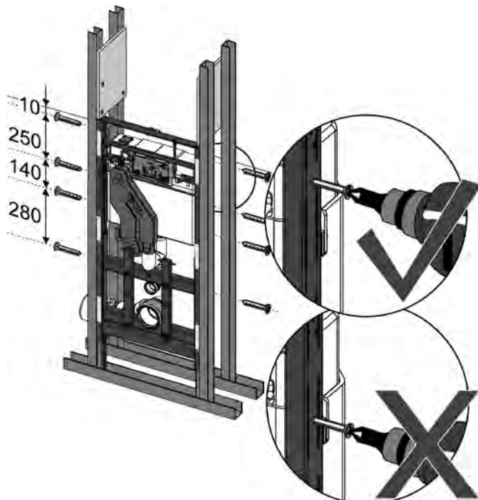
Securing the module during installation in a floor-to-ceiling C-profile steel post-and-beam wall system
