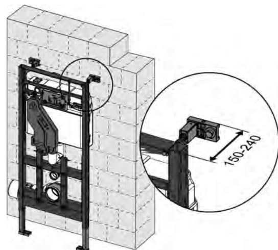
Adjustment range of the universal attachment 150 – 240 mm
