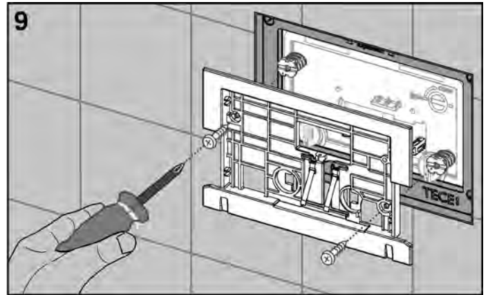
Screw the attaching frame onto the attaching rods.
