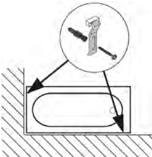
Securing the bathtub using bathtub anchors
