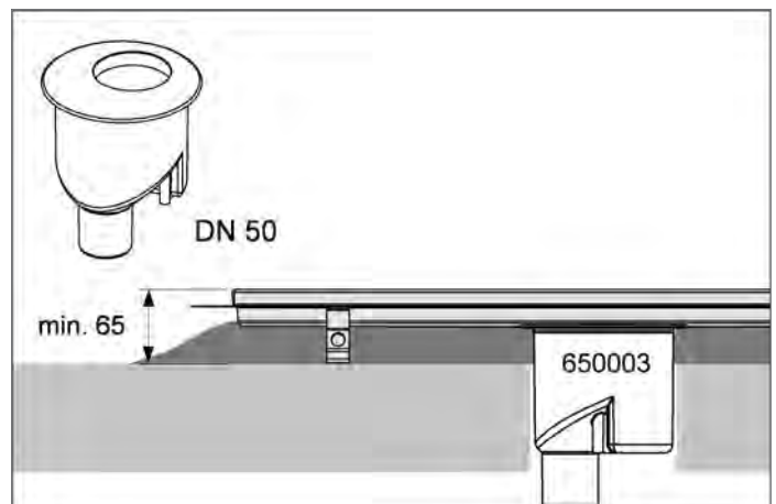
"Vertical" outlet
