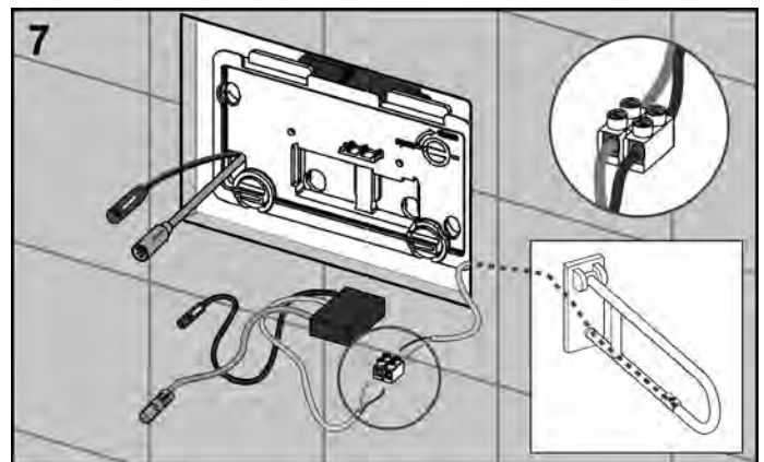
7 Install the splash guard with actuating motor. The actuation hooks must sit correctly in the lug of the drain valve. Tighten the attaching screws of the splash guard. Connect the cable from the button on the safety support arm to the electronic device (lustre terminal). Make sure the polarity is correct.
