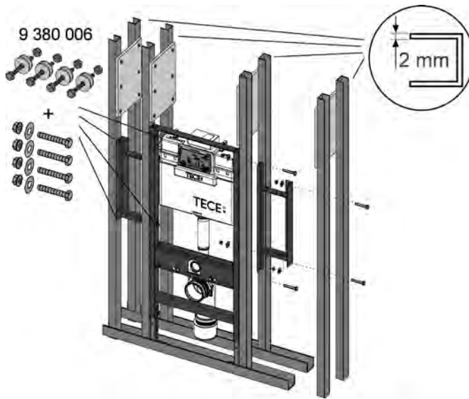
Installation in a steel post-and-beam wall
