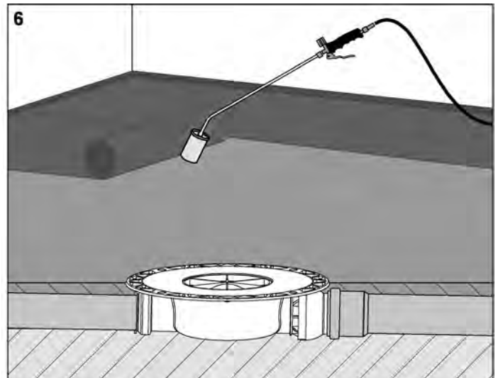
6 Apply sealing strips (bitumen/EPDM) in accordance with manufacturer information.
