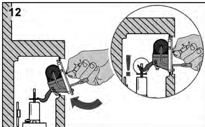
12 Insert the splash guard of the electronic device with actuating motor. The actuation hooks must sit correctly in the lug of the drain valve. Tighten the attaching screws of the splash guard.
