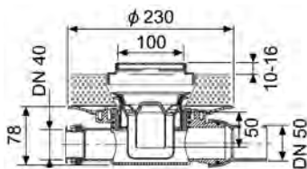
Floor drain horizontal, order number 685001
