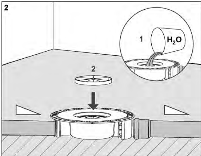
2 Carry out tightness test.
