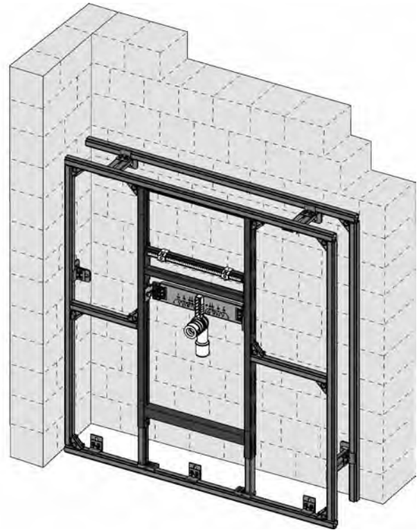
Modular construction with universal module for basin
