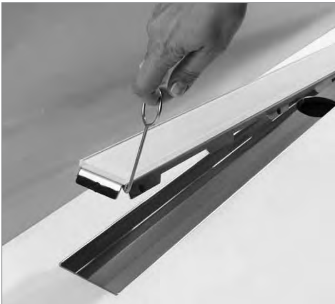
Remove the cover using the lifting tool
