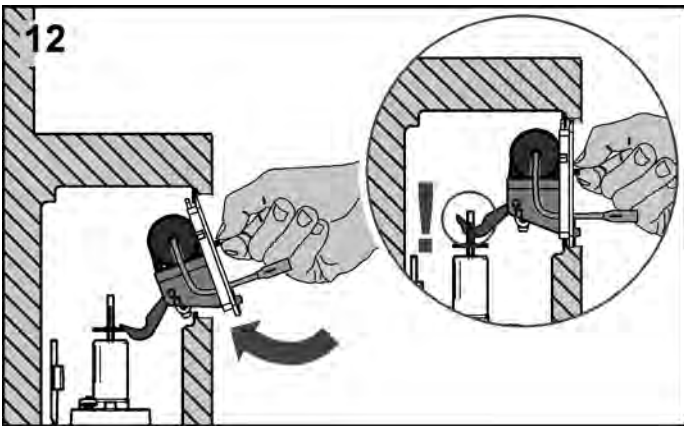
12 Insert the splash guard of the electronic device with actuating motor. The actuation hooks must sit correctly in the lug of the drain valve. Tighten the attaching screws of the splash guard.
