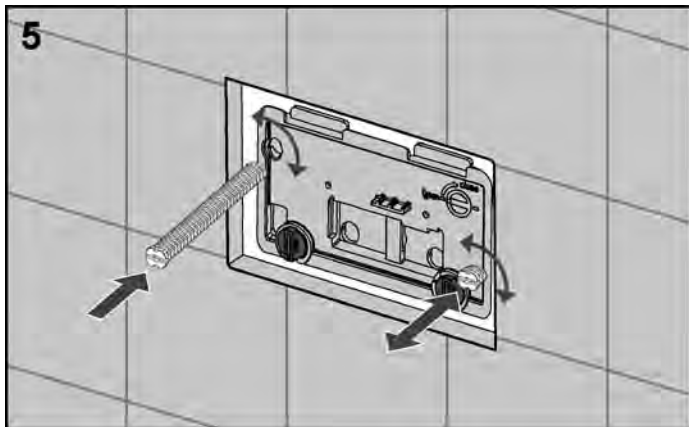
In the case of a two flush system, two actuation rods (red and blue) are installed. In a single flush system, only one is installed (blue).
