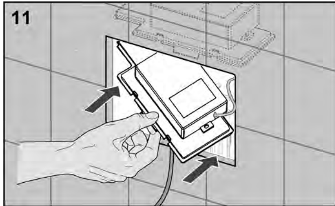
11 Place the electronic device and battery in the installation box, close this, and install it in the cistern again.
