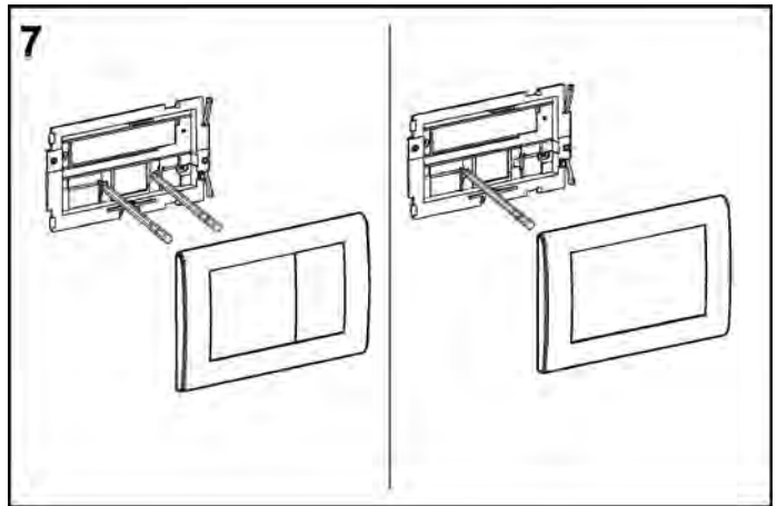
In the case of a two flush system, two actuation rods (red and blue) are installed. In a single flush system, only one is installed (blue).
