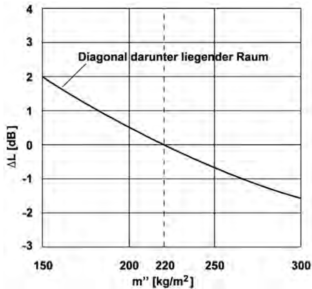
Change in the plumbing noise level – calculated results (calculated by the Fraunhofer Institute for Building Physics, Stuttgart)
