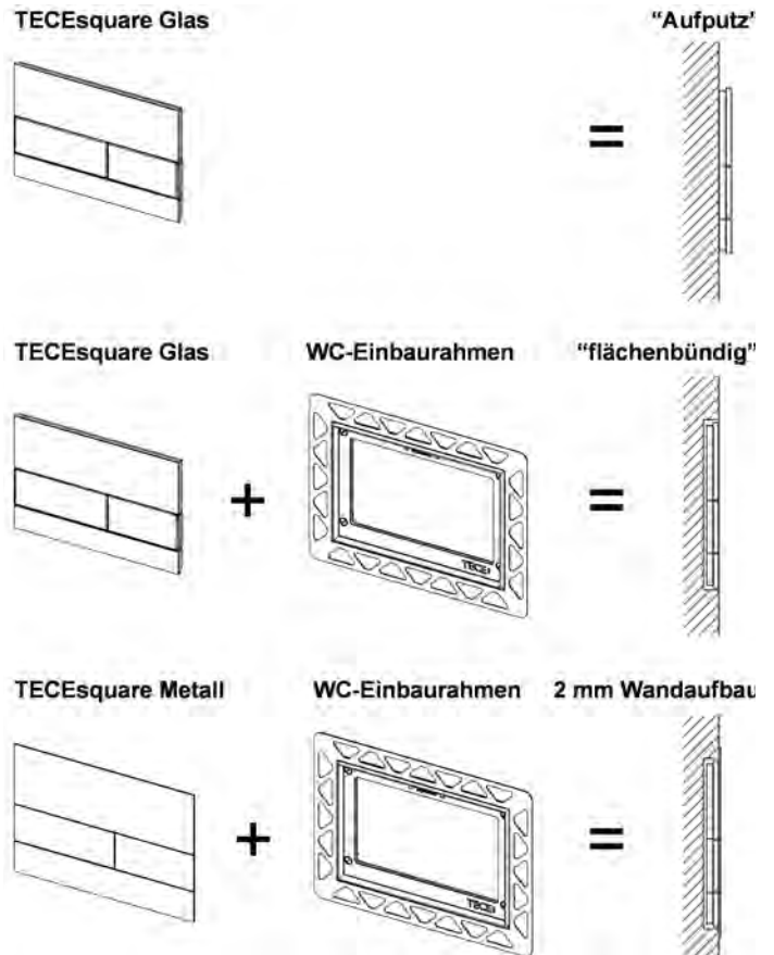
Installation of the TECEsquare push plates (for toilet and urinal push plates)
