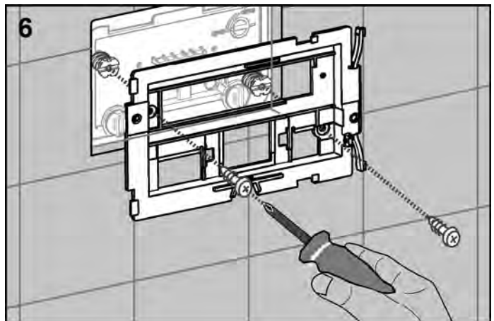
Install the attaching frame on the actuation rods.
