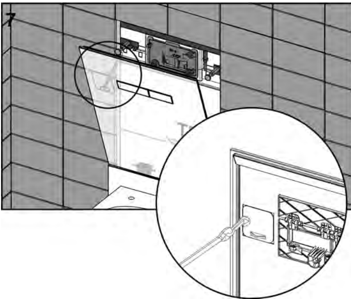
Secure the glass plate with security tape (engage the snap hooks into the eyes).
