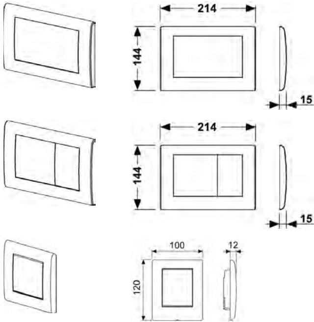
TECEplanus toilet push plate, single flush system TECEplanus toilet push plate, dual flush system TECEplanus urinal push plate
