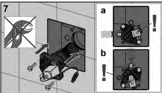
Install the electric cartridge (do not use tools to insert it!) and tighten the screws finger-tight.
