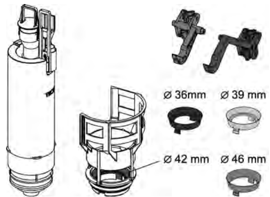
Conversion set 9 820 223, scope of delivery
