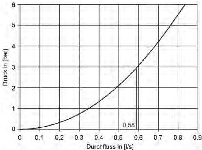
Flow diagram urinal electronics
