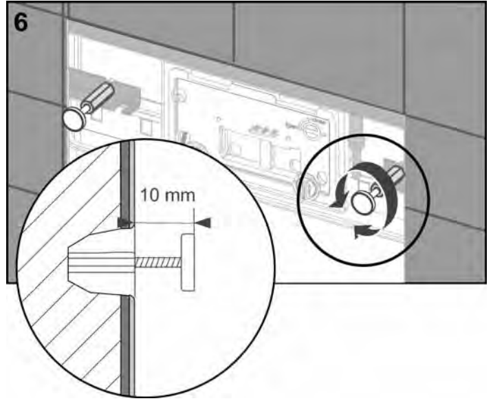
Screw in both securing magnets – 10 mm from wall surface.
