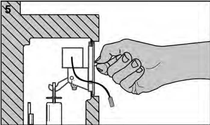
Insert the splash guard with electric actuation motor (supplied with the glass plate). No modification of the drain valve needed.
