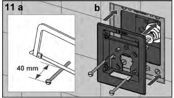
Screw the attaching frame to the urinal flush valve housing. If necessary, shorten the two screws so that they do not strike the mounting crossbeam (minimum length with minimum wall thickness = 40 mm).
