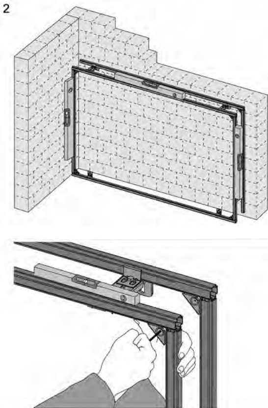
Use a spirit level to align the profiled tube and connect using corner joints
