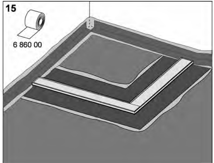
Apply sealing tape bubble-free.
