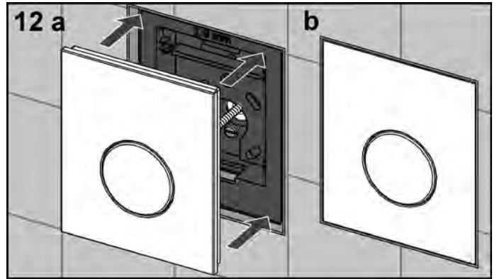
Snap the cover of the TECEloop push plate into the attaching frame.
