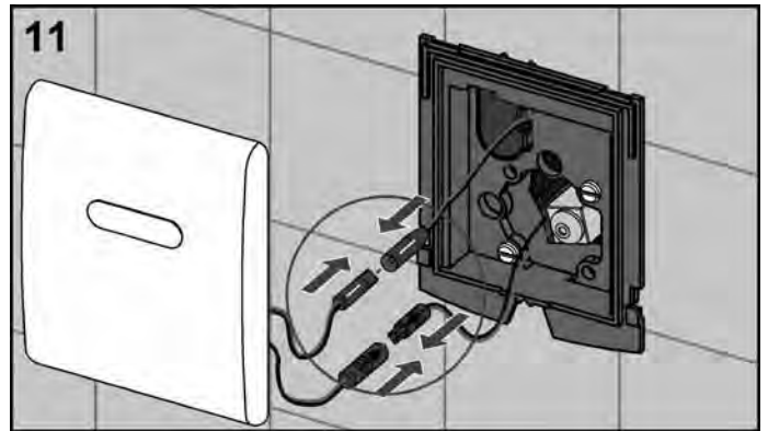
Connect the battery and the cartridge with the electronics.
