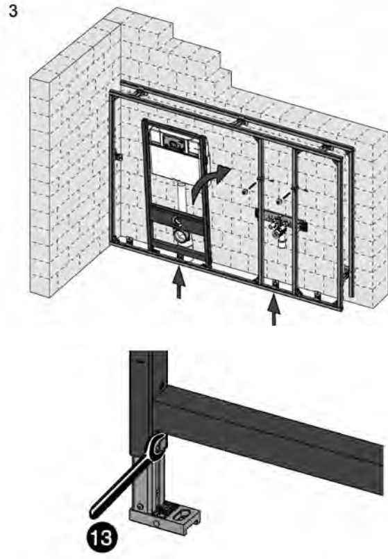
Place the angle bracket centred on the module or crossbeam, put the module feet onto the profiled tube, release the foot brake
