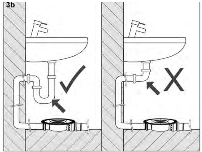
If a lateral inflow is used, an odour trap is required in the inlet pipe.
