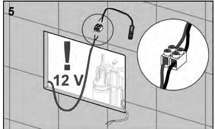
5 Connect the cable from the transformer to the network connection adapter (make sure the polarity is correct, see detail figure 5).
