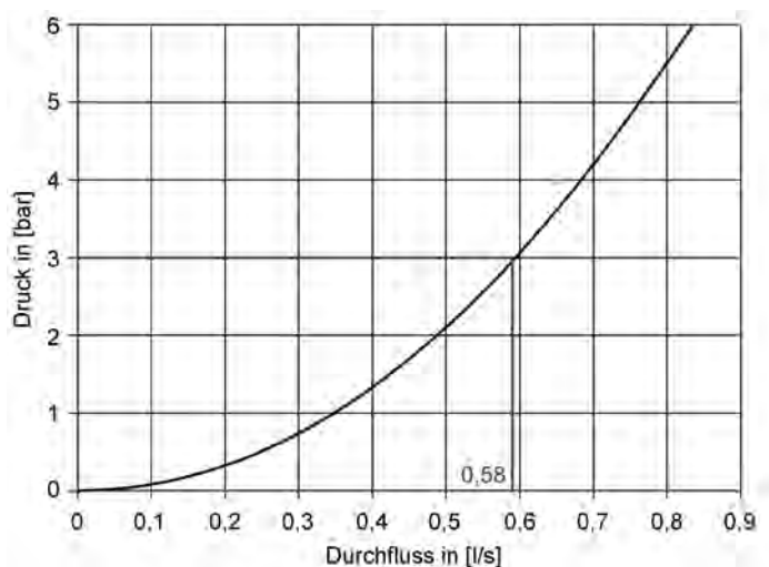
Urinal flow graph
