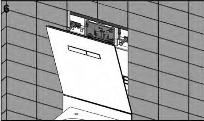
Insert the upper push plate into the brackets.
