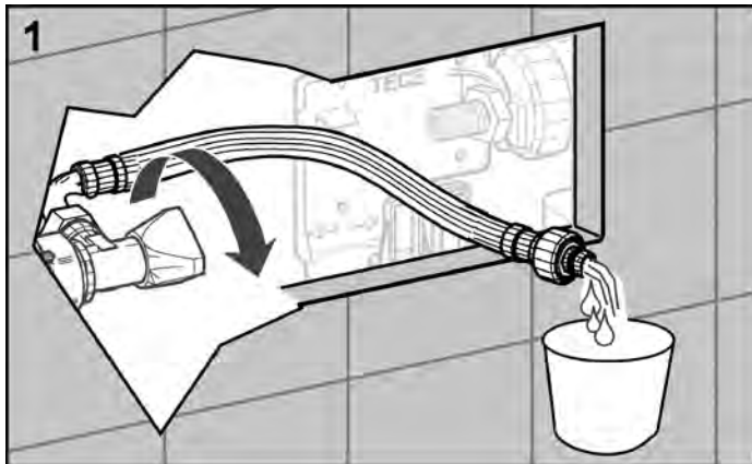
Open the corner valve and rinse out the pipe thoroughly.
