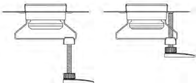
Height-adjustment facility of the mounting feet
