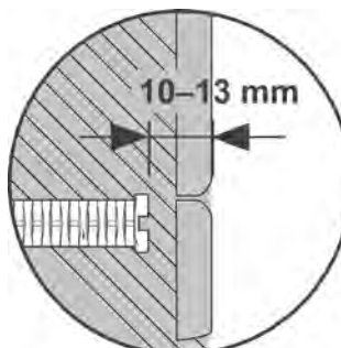
Screw in both attaching rods – distance between actuation rod and wall surface 10 to 13 mm.
