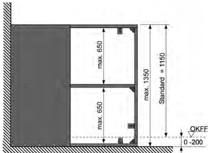
Dimensions of the facing sheets
