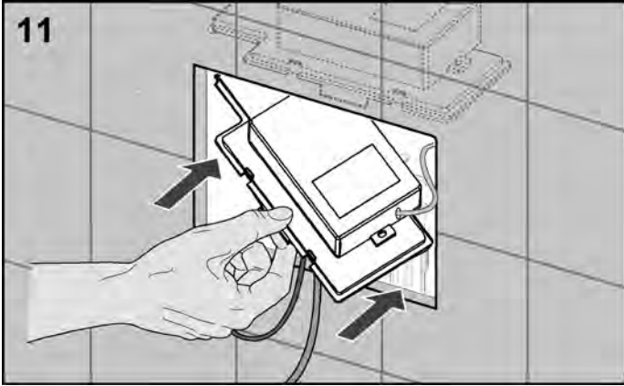
11 Place the electronic device in the installation box, close this, and install it in the cistern again.
