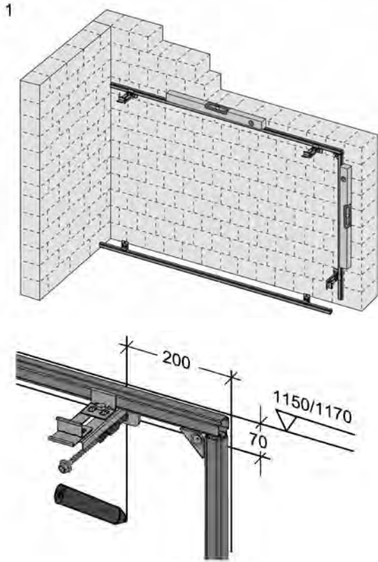
Secure the profiled tube to the wall with double brackets, to the floor with angle brackets
