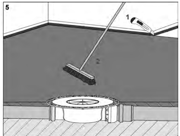
Once dry, cut off excess edge insulation strips and PE foil, clean screed.
