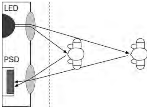
Function of the IR sensor with PSD technology
