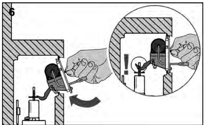
6 Guide the cable of the actuating motor through the opening in the splash guard.
