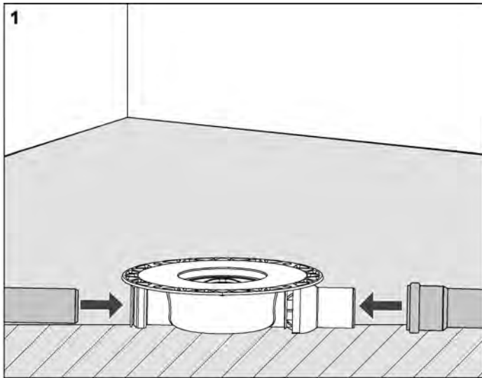
1 Position drain and connect on the waste-water side. In the case of drains with a vertical socket, a drill hole with a diameter of 130 mm is required.
