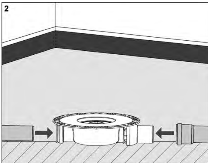
Position drain and connect on the waste-water side. In the case of drains with a vertical socket, a drill hole with a diameter of 130 mm is required.
