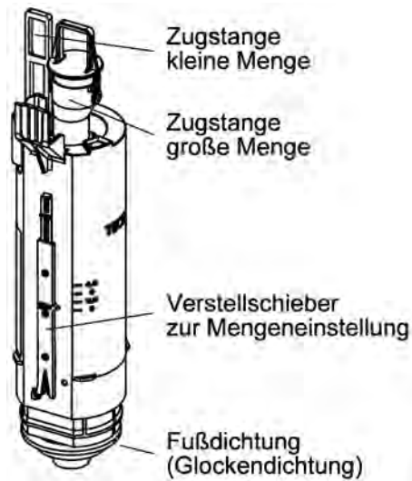
Drain valve A2, important components
