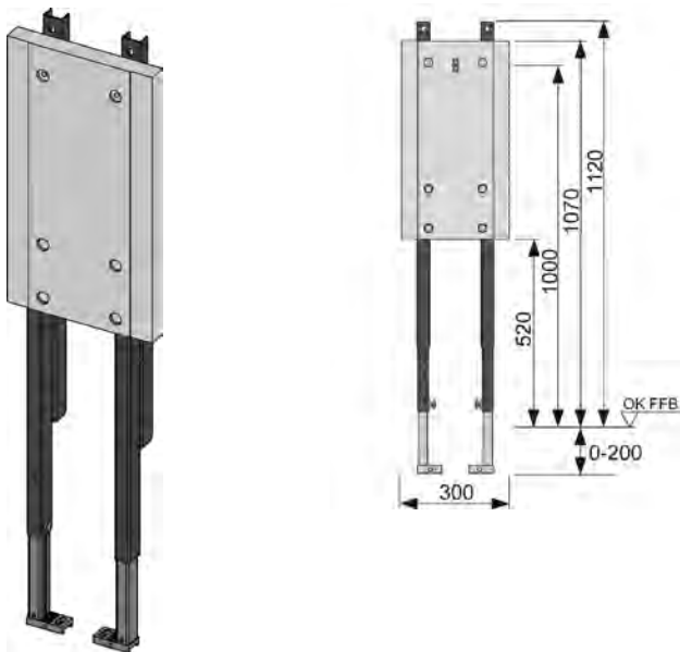
Module for handrail and support system (9 360 000)
