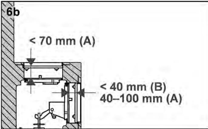
Snap off the actuation rods in accordance with the wall thickness.
