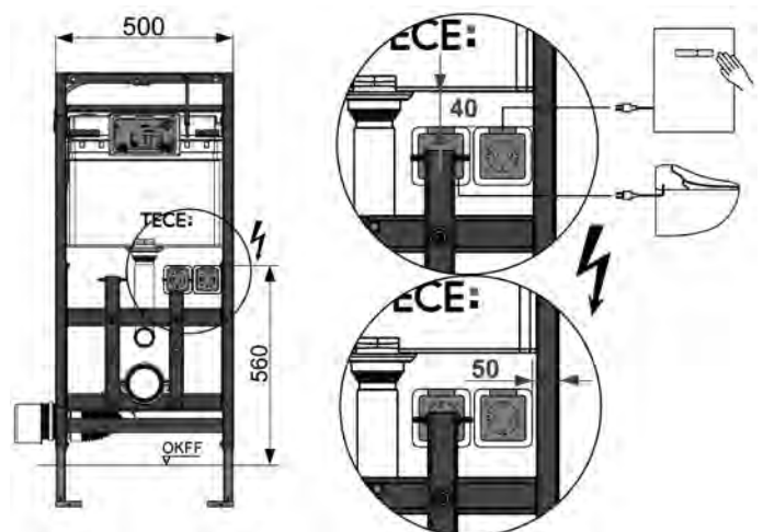
Positioning the socket(s) for the TECElux module
