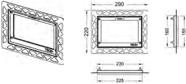
Flush-mounted installation frame for toilet push plate
