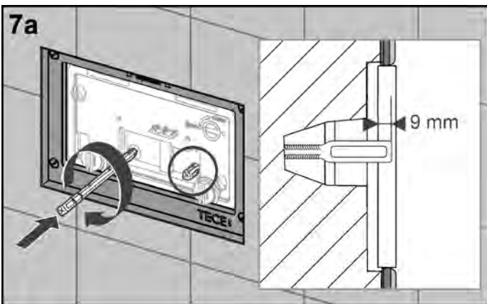
Screw in the actuation rods, set the distance to the front edge of the inner frame to 9 mm.
