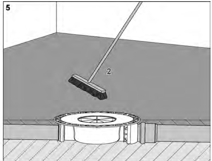
5 Once dry, clean the screed.
