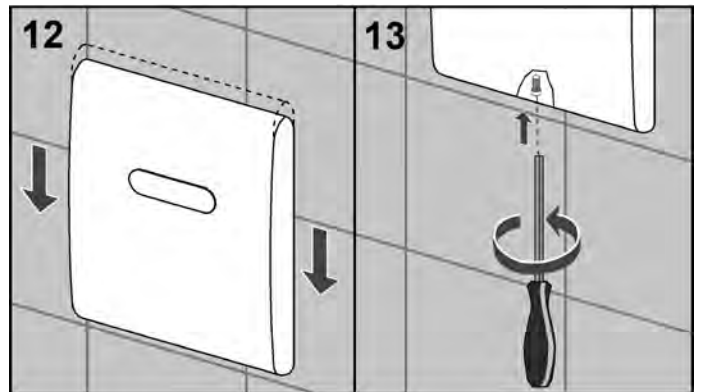
Finally install the cover of the push plate and install the supplied anti-vandal protection.
