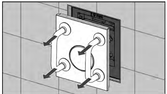
The installed cover can be removed from the actuation unit using the bow-type handles contained in the installation frame delivery. Position the suction cups only on the cover to be removed.
