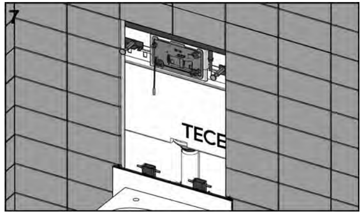
Screw in both securing magnets – 10 mm from wall surface.
