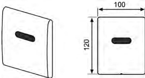
TECEplanus urinal electronic unit with infrared sensor
