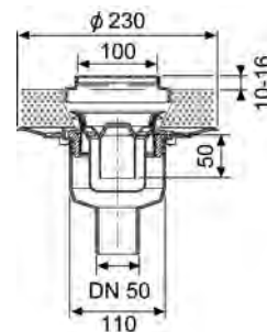
Floor drain vertical, order number 685000
