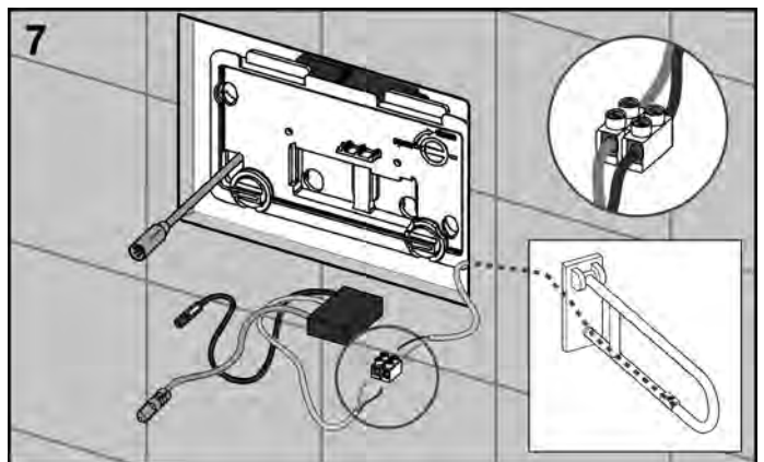
7 Connect the cable from the button on the safety support arm with the electronic device (lustre terminal). Make sure the polarity is correct.
