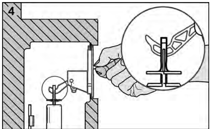
The actuation hooks must sit correctly in the lug of the drain valve. Tighten the attaching screws of the splash guard.
