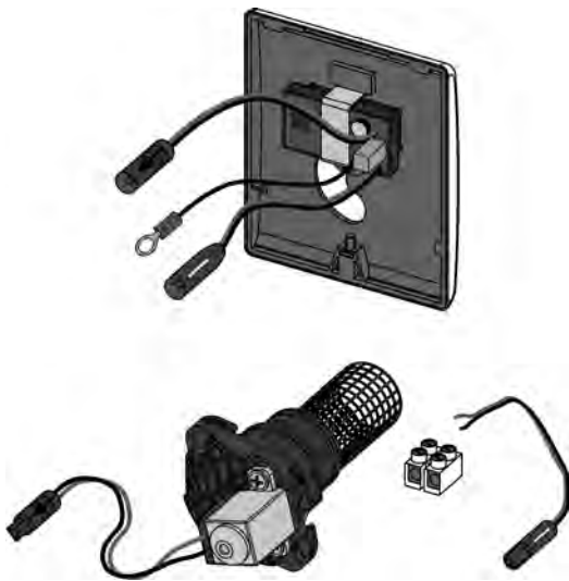
Urinal electronics, 230 V / 12 V mains version
