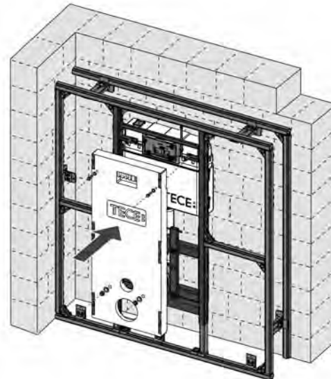
Secure bare-wall protection system on the module
